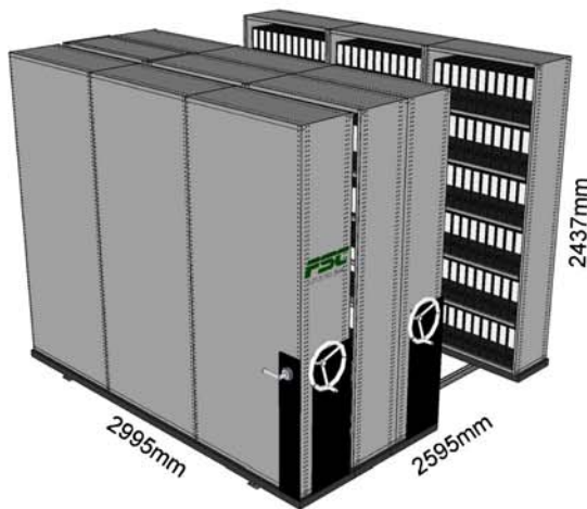
Heavy Duty Mobile Shelving 3 Wide 4 Bay System (7.8m 2 )*
